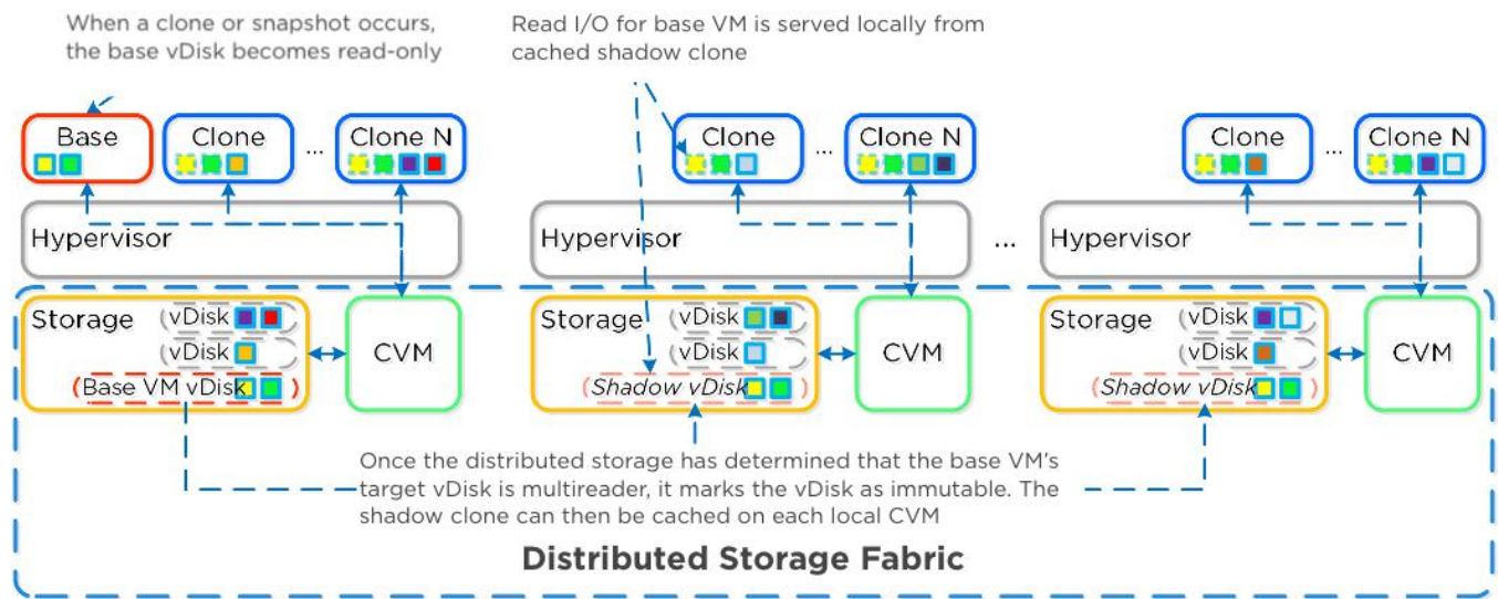
Figure 14: Nutanix Shadow Clones
