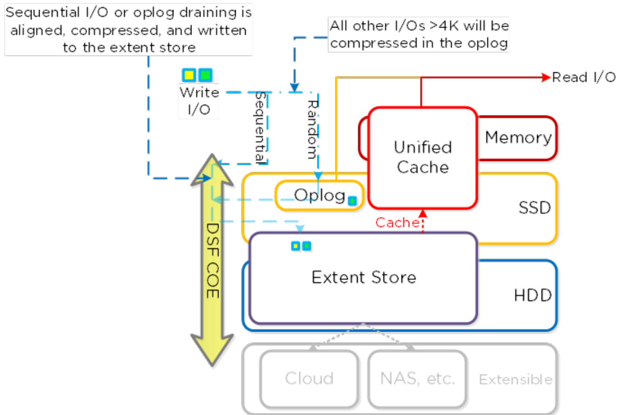
Figure 6: Inline Compression I/O Path
