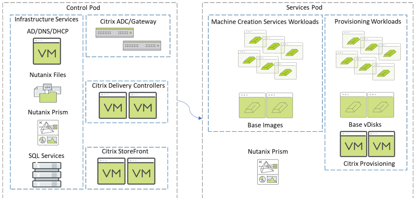
Figure 2: Virtual Apps and Desktops Pod Overview
