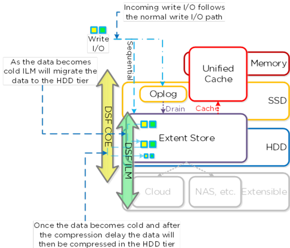
Figure 7: Post-Process Compression I/O Path
