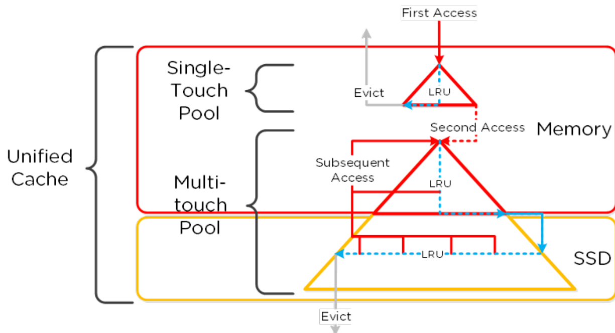
Figure 13: Unified Cache Data Path
