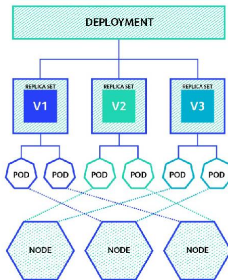
Figure V.4 : Deployments
