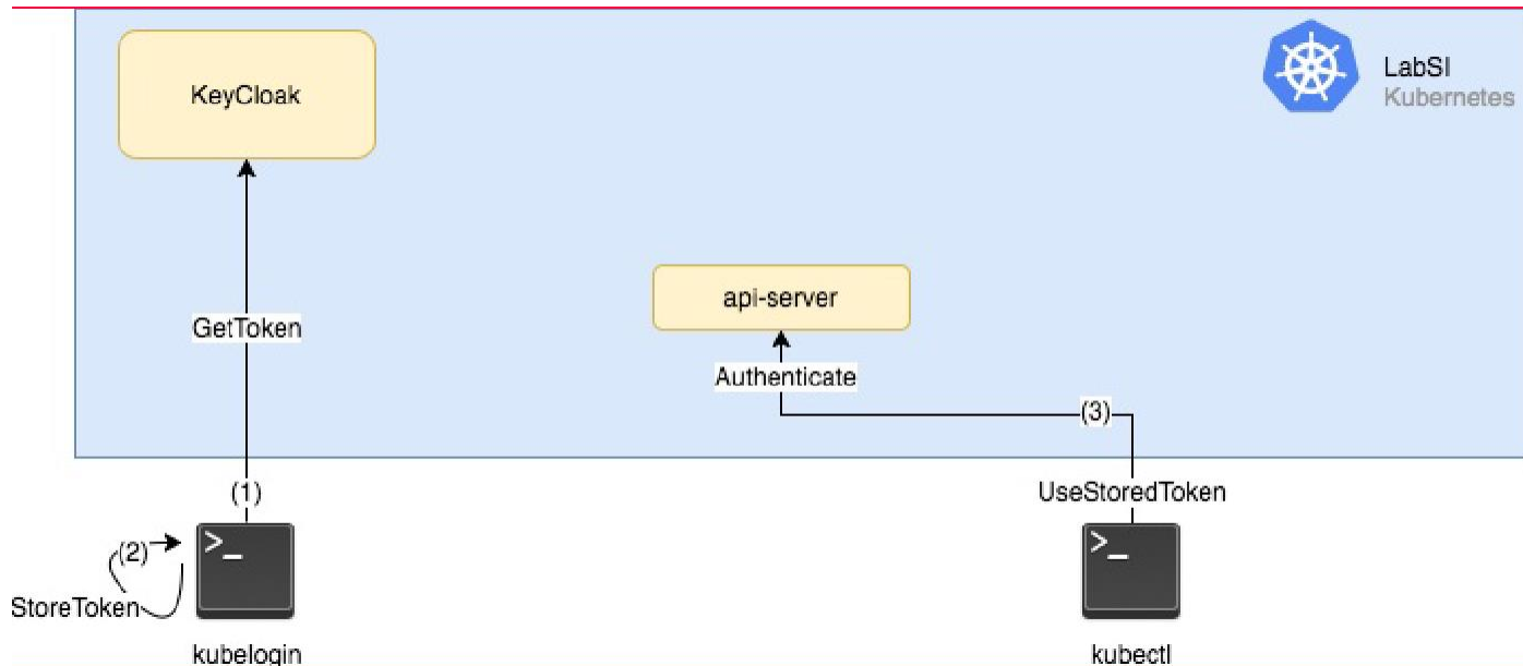
Figure VIII.4 : Authentification OIDC
